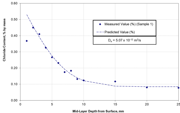
FIG 1: Example of ASTM C 1556 results with measured chloride values, the curve fit according to Fick's Second Law (dashed line), and the apparent diffusion coefficient ( D_a ).
