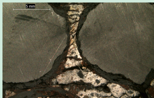
Stereo-optical micrograph of polished cross sectioned core showing corrosion and corrosion induced cracking of steel rebar.
