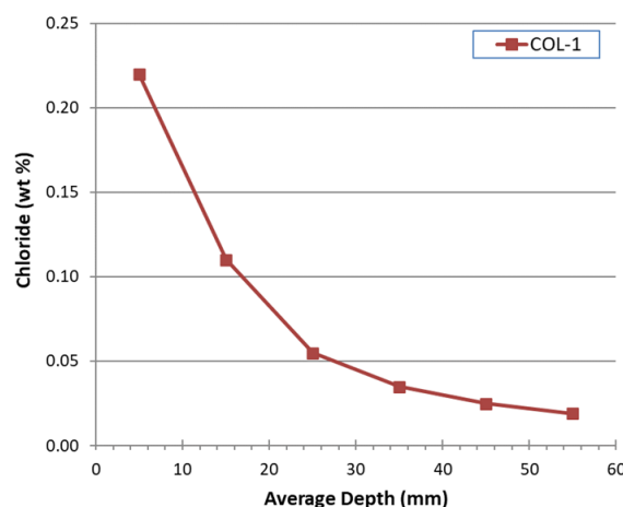
Fig 2: Example of chloride profile with ASTM C1152 testing at 10-mm depth intervals.
